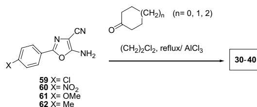
Scheme 5. Synthesis of tacrine-analogues 30–40 by Friedländer reaction.
