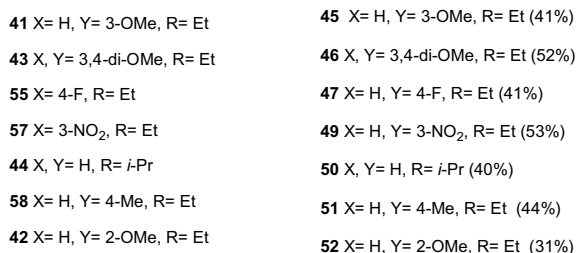
Scheme 4. Synthesis of pyridines 45–47 , 49 and 50–52 .
