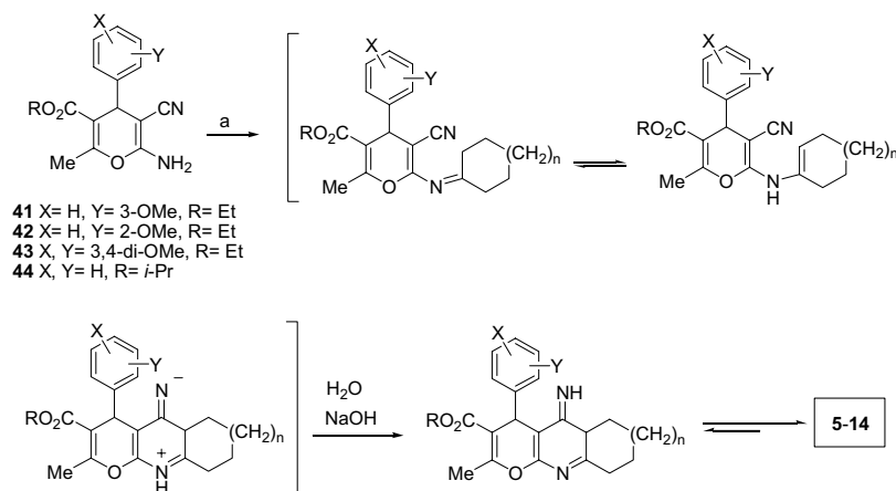
Scheme 2. Synthesis of tacrine-analogues 5–14 by Friedländer reaction. Reagents and conditions: (a) cyclopentanone ( n = 0 ), cyclohexanone ( n = 1 ), cycloheptanone ( n = 2 ), (\text{CH}_2)_2\text{Cl}_2 , \text{AlCl}_3 , reflux.
