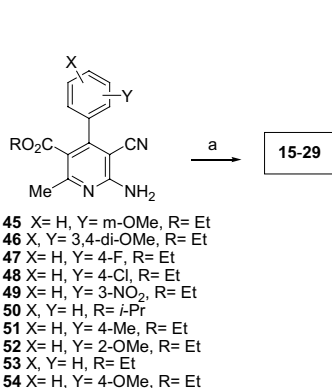
Scheme 3. Synthesis of tacrine-analogues 15–29 by Friedländer reaction. Reagents and conditions: (a) cyclohexanone ( n = 1 ) or cycloheptanone ( n = 2 ) or cyclooctanone ( n = 3 ), (\text{CH}_2)_2\text{Cl}_2 , \text{AlCl}_3 , reflux.
